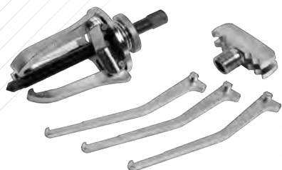
26Q4-CJ250 13 PC MEDIUM-DUTY GENERAL PURPOSE PULLER SET
