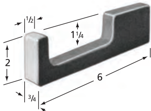
ATI760B-3 1.75 LBS
