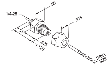
ATI503C-1/8
